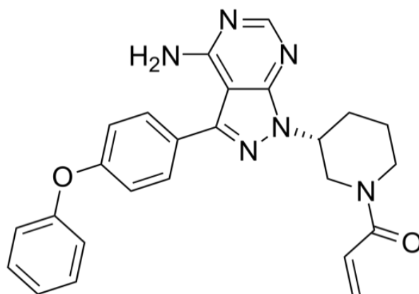
Fig 1: Chemical Structure of Ibrutinib
