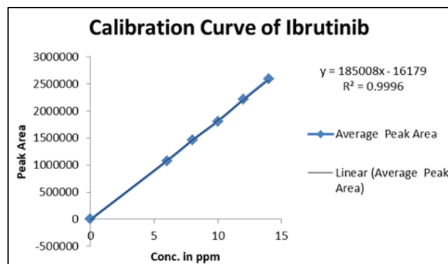
Fig 3: Linearity Curve of Ibrutinib
